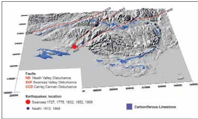
A view of the South Wales Coalfield showing the distribution of the Carboniferous Limestone, the positions of the three major disturbances and their association with the history of earthquakes in south Wales since the early 18th century.
