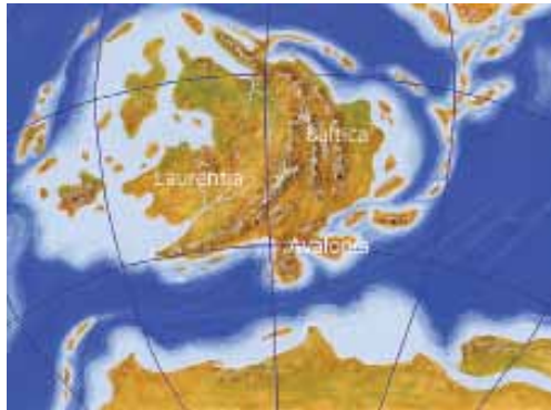
Devonian palaeomap.
